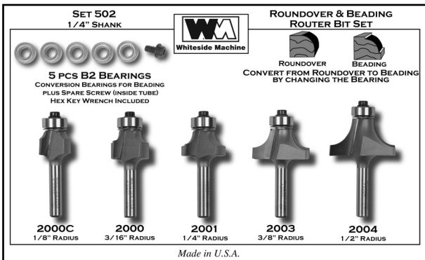
Set 502 - ROUNDROVER & BEADING - 1/4" Shank
