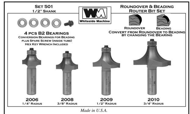
Set 501 - ROUNDROVER & BEADING - 1/2" Shank
